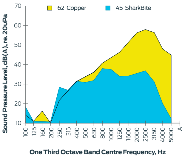
Measured noise level of water flow through nominal 15mm bore SharkBite and copper pipe, 20L/min, 600kPa with DIN 52218 noise source.
