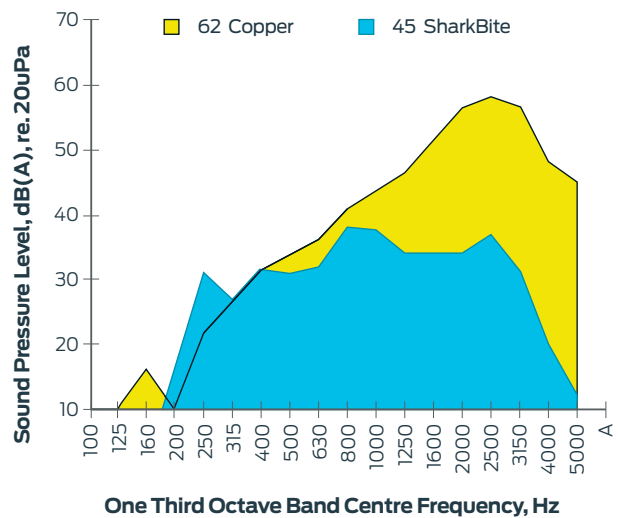
Measured noise level of water flow through nominal 15mm bore SharkBite and copper pipe, 20L/min, 700kPa with DIN 52218 noise source.
